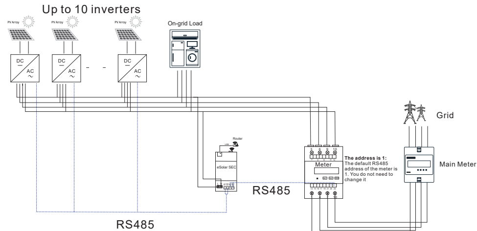
Fig 7: Parallel System Wiring
