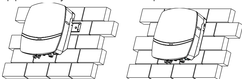
Figura 4.9 Monte R5-(0,7K, 1K, 1,5K, 2K, 2,5K, 3K)-S1-15 Inversor R5-(3K, 3,6K, 4K, 5K, 6K, 7K, 7,5K, 8K)-S2-15
